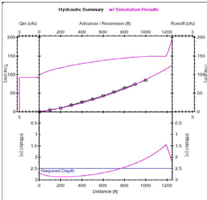
Figure 2. Summary of irrigation hydraulics for a germination irrigation at DREC.
